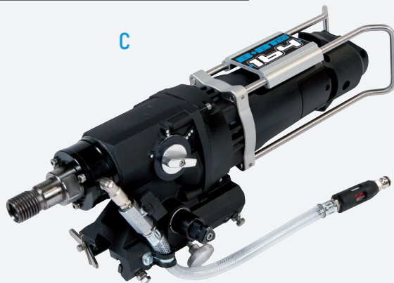
C Karat 164: Motor/Gearbox/Slide, complete. 2.000W for Bit Range Ø10 - Ø164 mm.
